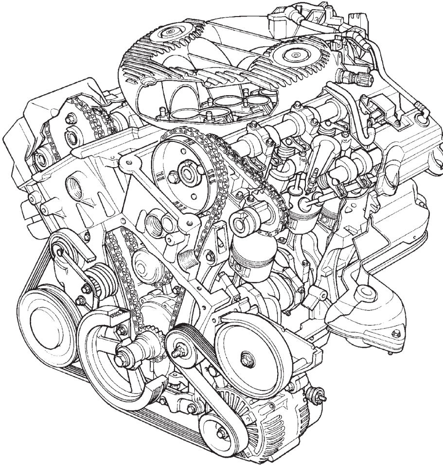
Fig. 1 2.7 Liter Engine
