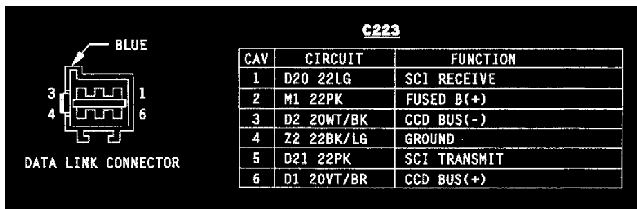
Data Link Connector
